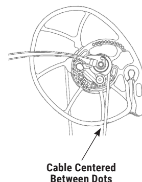
Figure 8: Cam Timing
