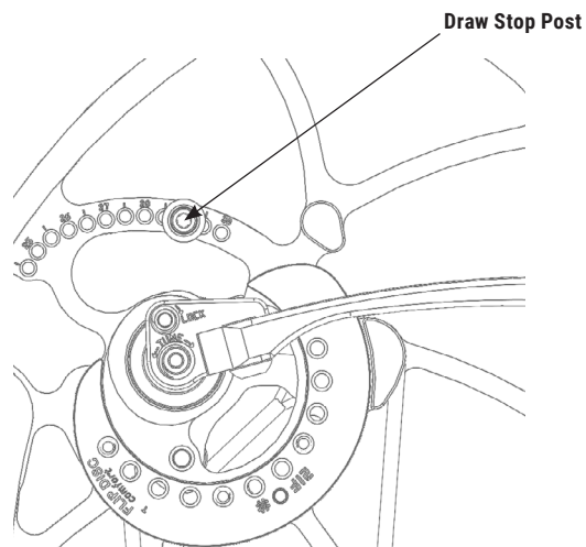
Figure 2: CP28 FlipDisc & Post Settings
