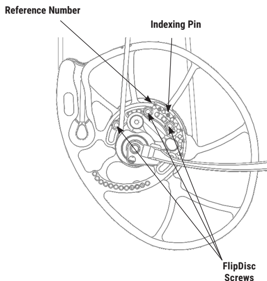
Figure 1: CP28 Series FlipDisc Settings
