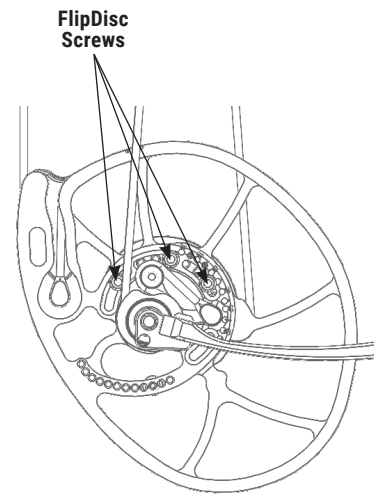
Figure 3: FlipDisc Adjustment
