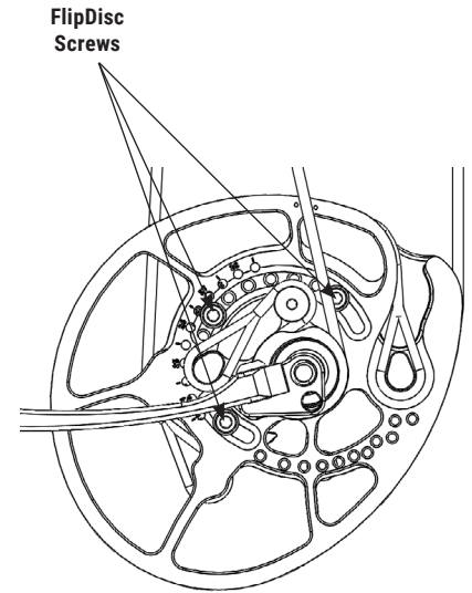
Figure 3: FlipDisc Adjustment
