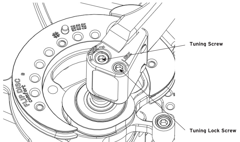
Figure 4: DeadLock Adjustment
