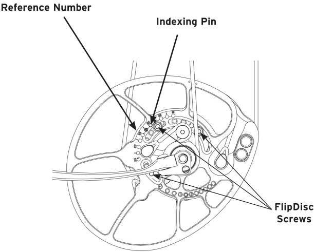
Figure 1: FlipDisc Settings
