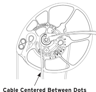
Figure 8: Cam Timing
