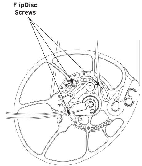
Figure 3: FlipDisc Adjustment
