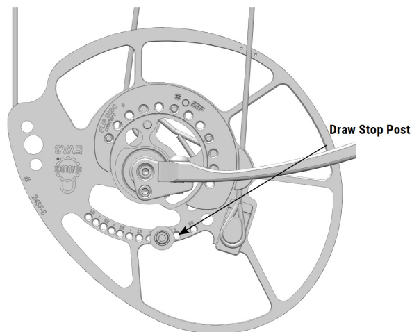
Figure 2: FlipDisc & Post Settings
