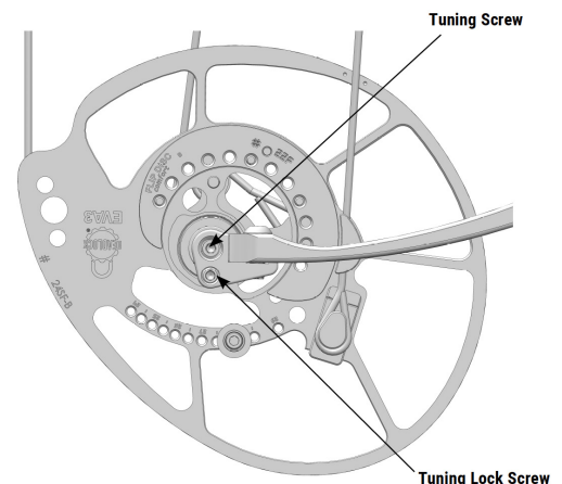
Figure 4: DeadLock Adjustment
