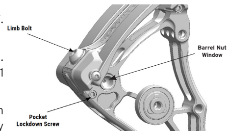
Figure 8: Draw Weight Adjustment
