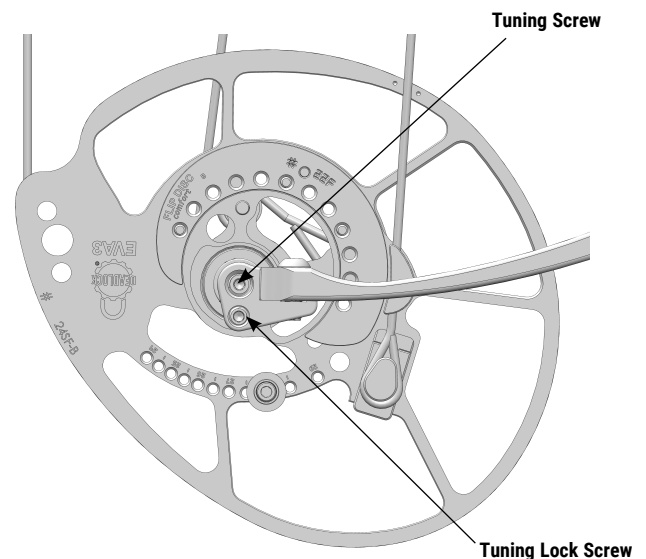
Figure 4: DeadLock Adjustment
