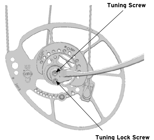
Figure 4: DeadLock Adjustment
