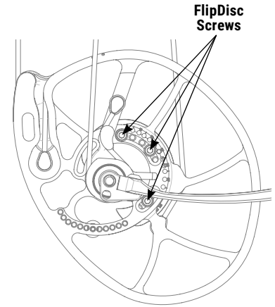
Figure 3: FlipDisc Adjustment
