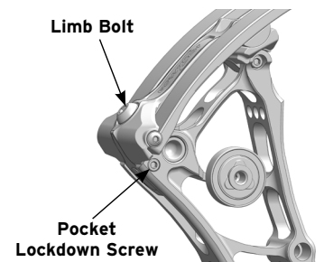
FIGURE 8: DRAW WEIGHT ADJUSTMENT
