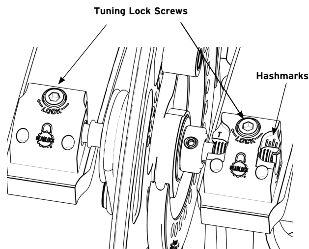
Figure 4: DeadLock Adjustment
